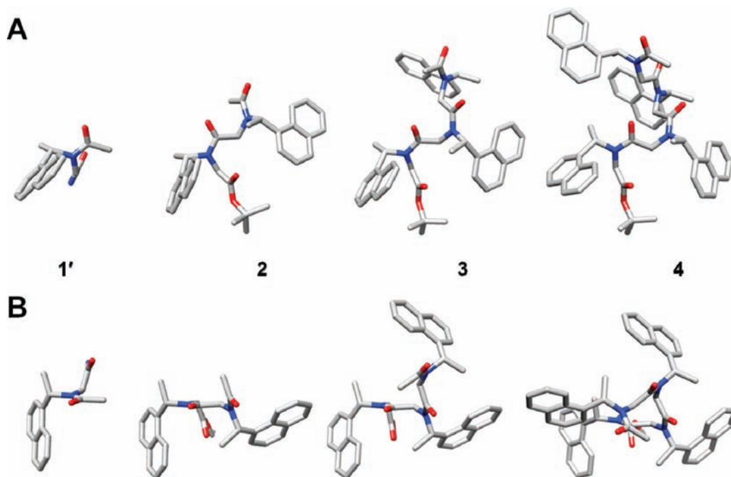
Figure 2. X-ray crystal structures of peptoids 1' and 2–4. (A) View perpendicular to the helical axis. (B) View parallel to the helical axis. Atom designations: red = oxygen; blue = nitrogen; gray = carbon. Hydrogen atoms in parts A and B and the t -butyl methyl groups in part B have been removed for clarity.
